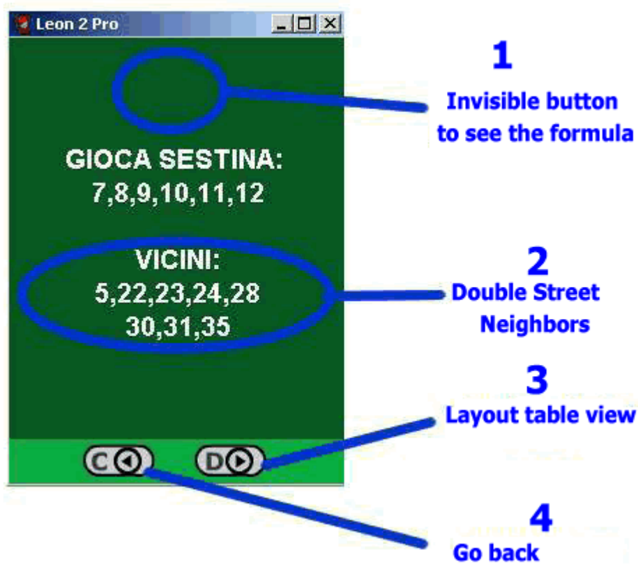
Neighbors Prediction
